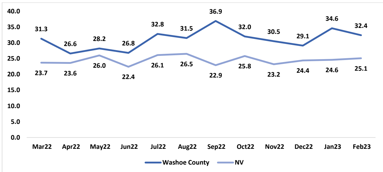
Figure 2. Monthly rates of suspected drug-related overdose ED visits in Washoe County vs NV, past 12 months (per 100,000 population)
